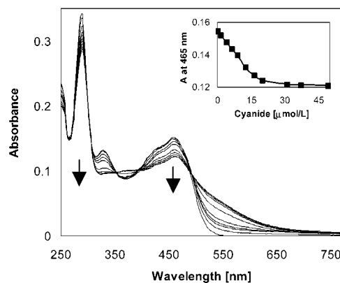
Figure 1. Changes in the UV-vis spectrum of sensor 1 (9.04 \mu\text{M} in \text{CH}_2\text{Cl}_2/\text{CH}_3\text{CN} (98:2)) upon the addition of cyanide (0–49.02 \mu\text{M} ). (Inset) Binding isotherm monitored by the absorbance decrease at 465 nm.
