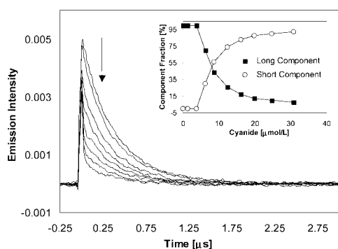
Figure 3. Changes in the time-resolved PL decay of sensor 1 ( 9.04 \mu\text{M} ) upon the addition of cyanide ( 0\text{--}32 \mu\text{M} ), obtained with 458 \text{ nm} excitation. (Inset) Shifts in fractional intensity of the two lifetime components obtained from biexponential analysis. See text for details.
