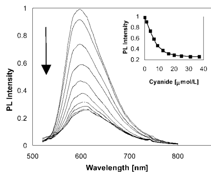
Figure 2. Changes in photoluminescence intensity of sensor 1 ( 9.04 \mu\text{M} ) in \text{CH}_2\text{Cl}_2/\text{CH}_3\text{CN} (98:2) upon the addition of cyanide ( 0\text{--}38.79 \mu\text{M} ). (Inset) Binding isotherm monitored by the integrated luminescence intensity. \lambda_{\text{ex}} = 493 \text{ nm} (isosbestic point in UV-vis spectra).
